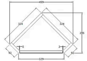
NVC118 - CORNER MIRROR CABINET
